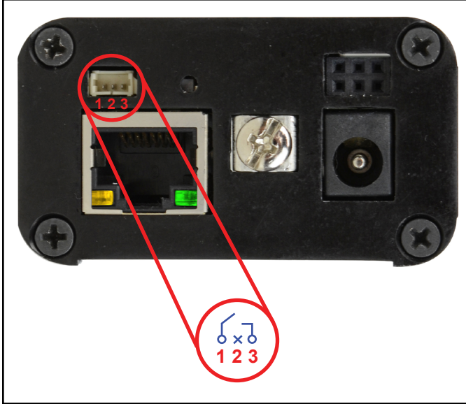
Figure 8. Relay terminal pin-out
