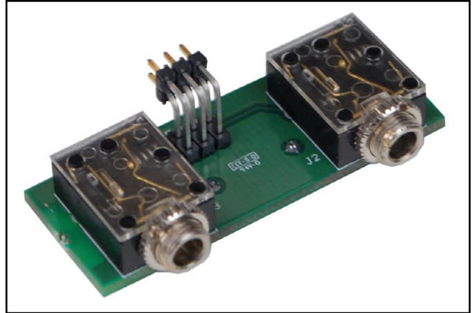
Figure 10. SCS CTA245 Replacement Wrist Strap Jack PCB for the WS Aware Monitor
