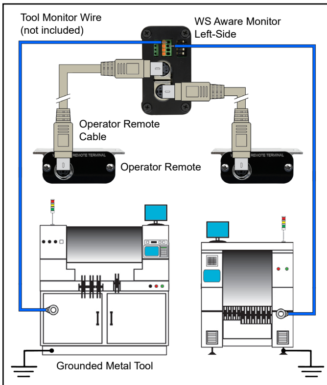
Figure 6. Wiring the WS Aware Monitor to two metal tools
