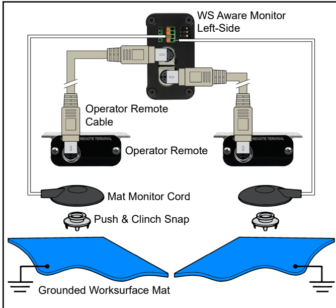
Figure 5. Wiring the WS Aware Monitor to two workstations
