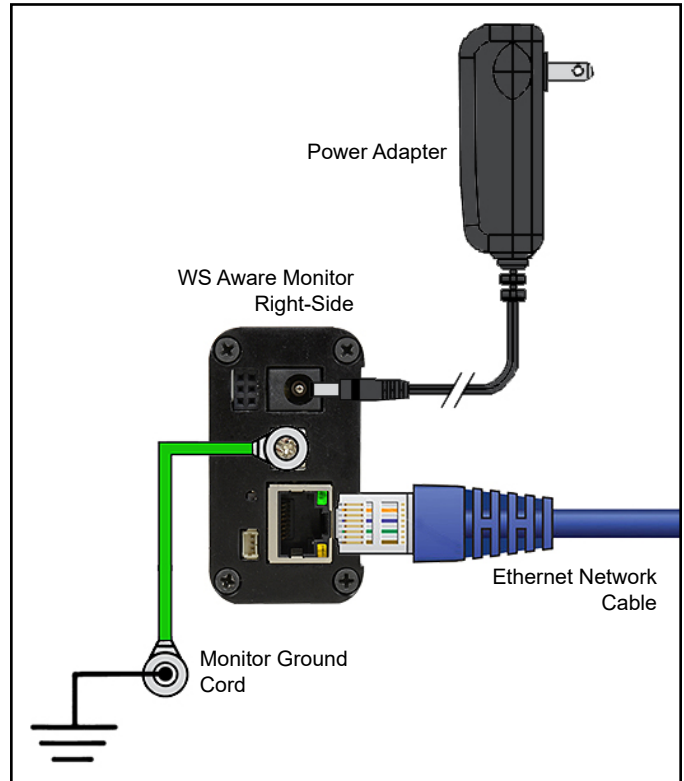
Figure 7. Connecting the WS Aware Monitor to ground, Ethernet and power.
