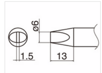
T33-D6 Shape-6D
