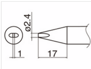
T33-D24 Shape-2.4D
