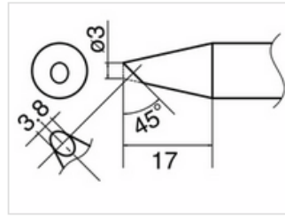
T33-BC3 Shape-3BC
