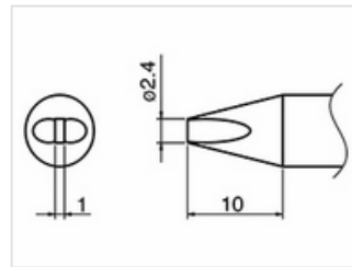
T33-SSD24 Shape-2.4SSD
