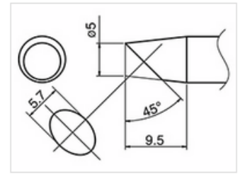
T33-SSBC5 Shape-5SSBC
