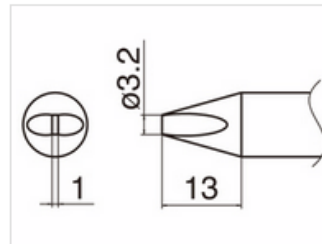
T33-D32 Shape-3.2D
