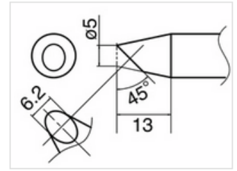
T33-BC5 Shape-5BC
