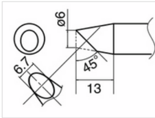
T33-BC6 Shape-6BC
