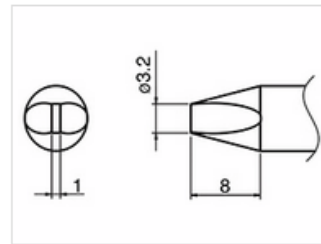
T33-SSD32 Shape-3.2SSD
