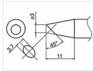
T33-SSBC3 Shape-3SSBC
