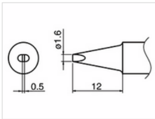
T33-SSD16 Shape-1.6SSD
