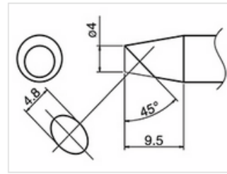
T33-SSBC4 Shape-4SSBC
