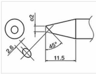
T33-SSBC2 Shape-2SSBC
