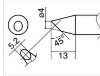
T33-BC4 Shape-4BC
