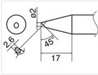
T33-BC2 Shape-2BC
