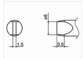
T33-SSD6 Shape-6SSD
