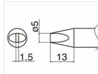
T33-D5 Shape-5D
